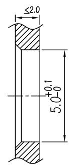
Panel cut-out
